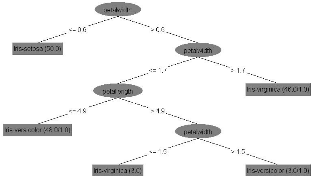
Fig. 5.4 : Visualization of a decision tree on the Fisher iris dataset
