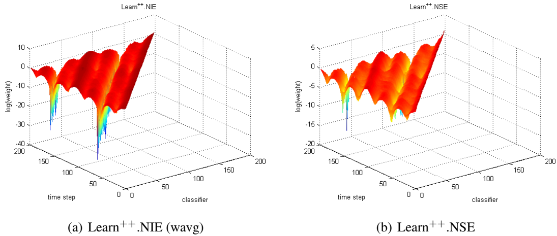
Fig. 5.11 : Learn ++ weight evolution on Gaussian concept drift problem
