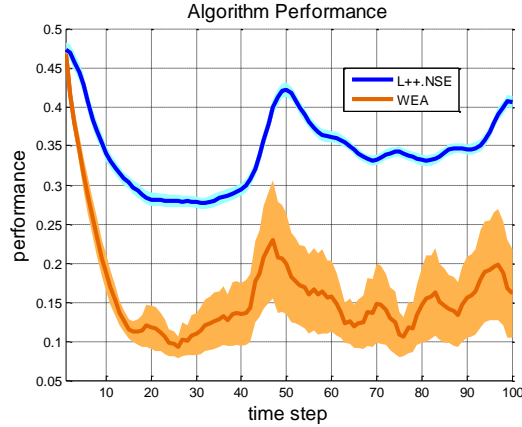
Fig. 5.39 : WEA vs. Learn ++ .NSE on Rotating Circular Gaussian Drift with Failure
