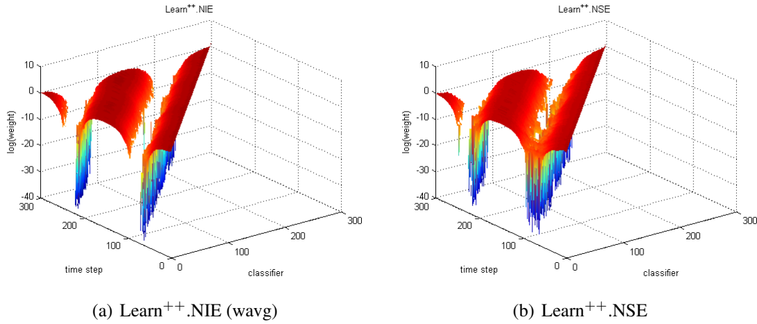
Fig. 5.17 : Learn ++ weight evolution on Spiral Data
