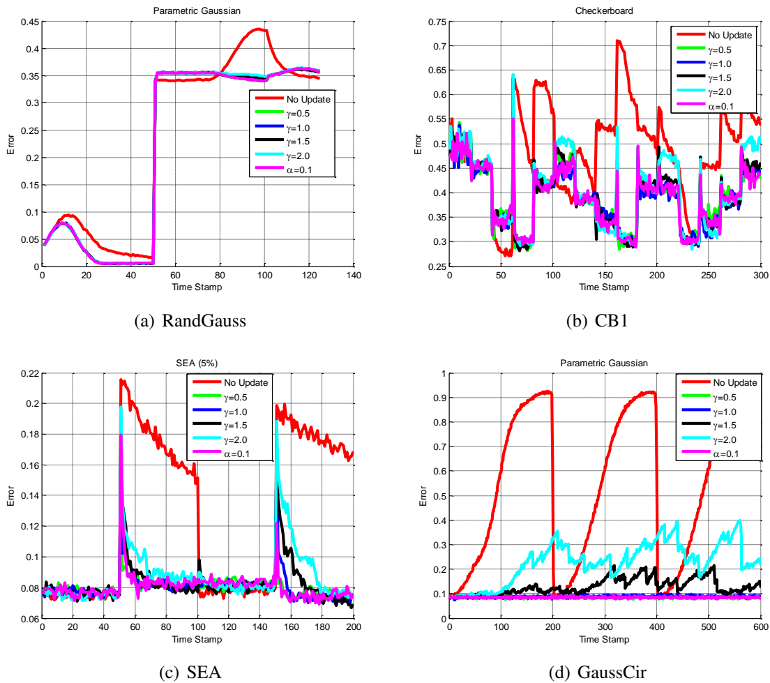
Fig. 5.47 : Error evaluation of the on-line naïve Bayes classifiers (updated and dynamically reset) with a variation in the parameters of the Hellinger Distance Drift Detection Method (HDDDM).
