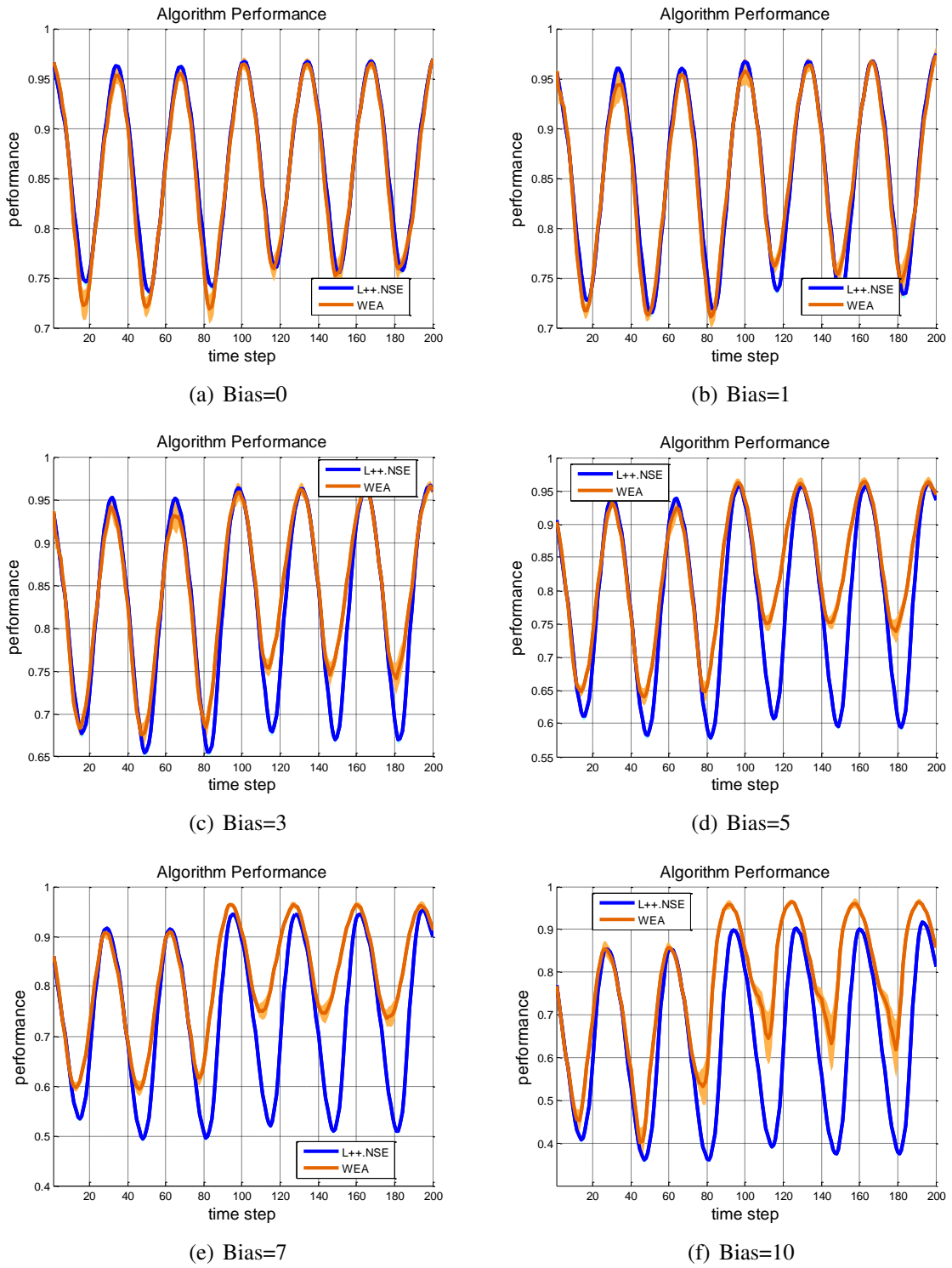
Fig. 5.40 : WEA vs. Learn ++ .NSE on Rotating Triangular Gaussian Drift
