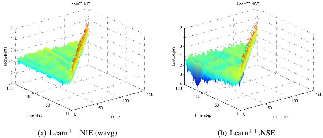
Fig. 5.37 : Learn ++ weight evolution on NOAA
