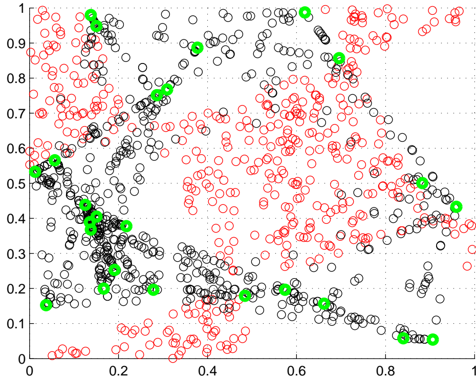
Fig. 3.10 : SMOTEs generation of synthetic minority class instances in the regions of the majority class feature space, thus leading to the degradation of the overall accuracy of a classifier. Green instances represent are the original minority class instances, red are the majority class instances, and black are the synthetic instances.
