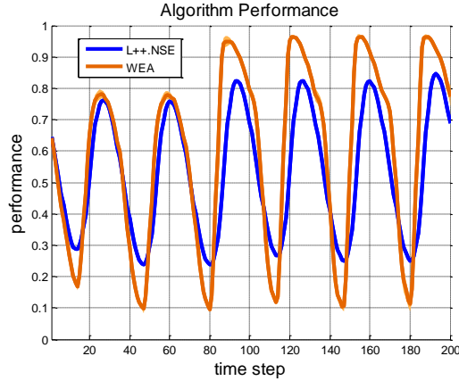
Fig. 5.41 : WEA vs. Learn ++ .NSE on rotating triangular Gaussian drift with 13 time stamp bias.
