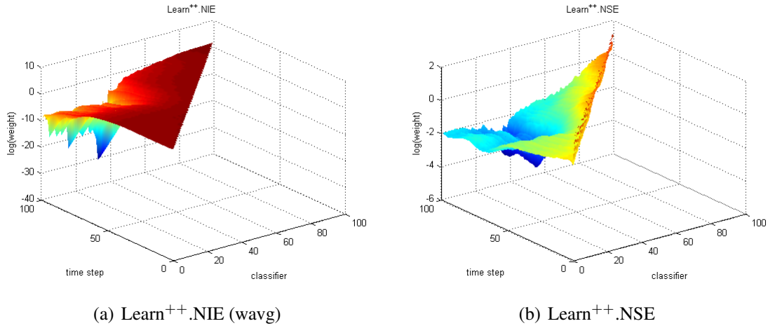
Fig. 5.22 : Learn ++ weight evolution on Gaussian concept drift problem
