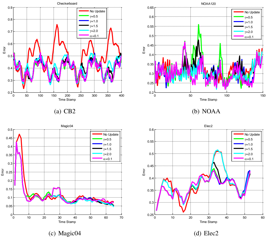
Fig. 5.46 : Error evaluation of the on-line naïve Bayes classifiers (updated and dynamically reset) with a variation in the parameters of the Hellinger Distance Drift Detection Method (HDDDM).
