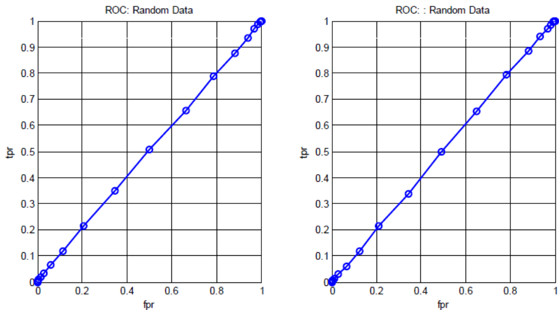
Fig. 5.2 : A naïve Bayes classifier with a Gaussian kernel was generated on 10,000 random instances drawn from a standardized Gaussian distribution. The class labels are produced by computing the \text{sign}(\mathcal{N}(0,1)) . The AUC for \omega_1 (left) is 0.50185 and \omega_2 (right) is 0.50295.
