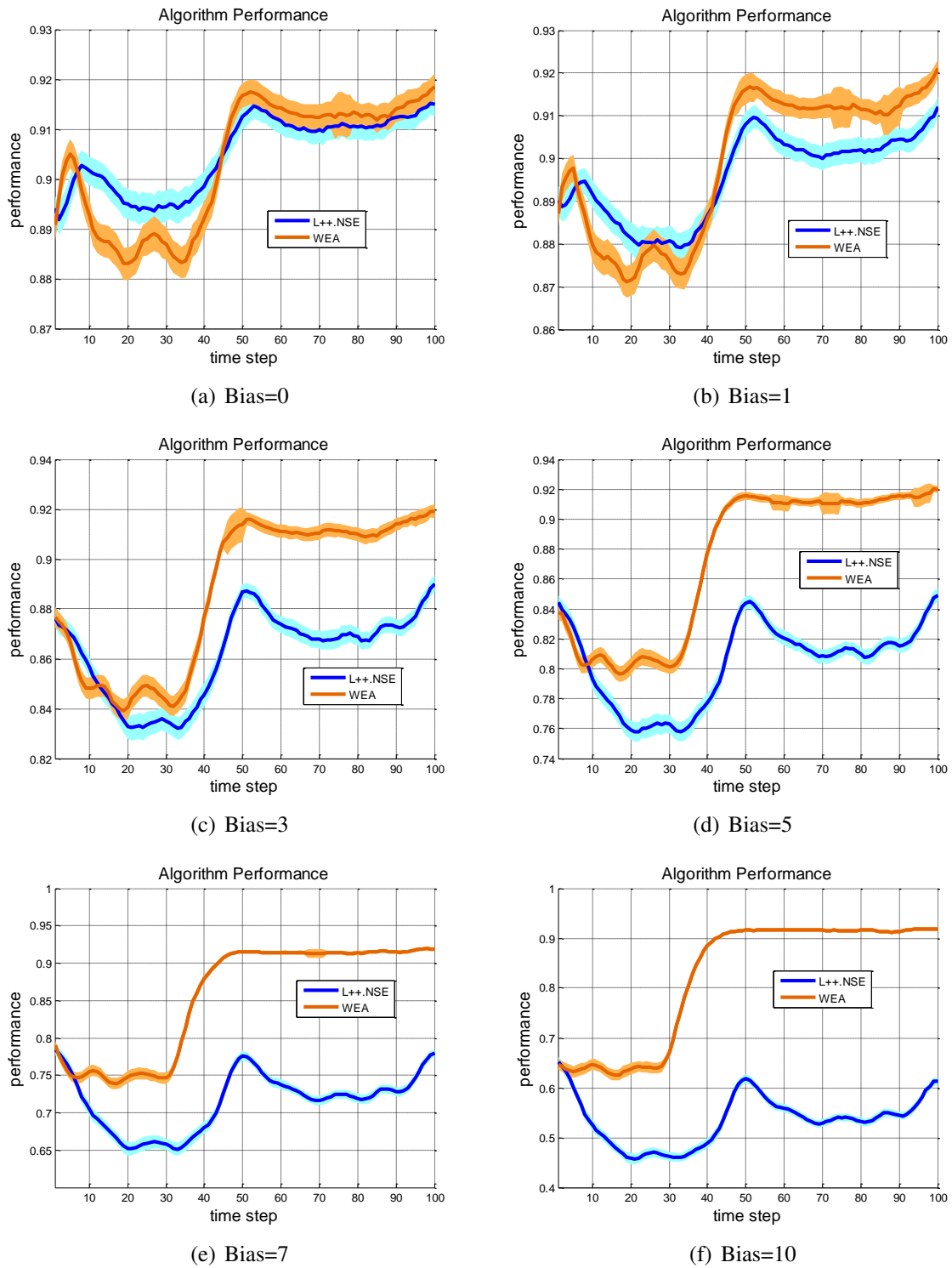
Fig. 5.38 : WEA vs. Learn ++ .NSE on Rotating Circular Gaussian Drift
