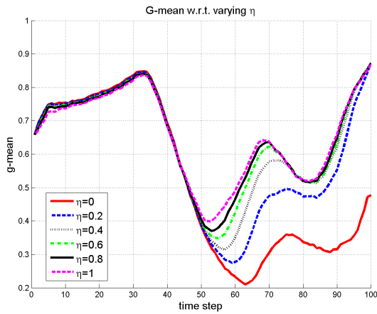
(c) G-mean
