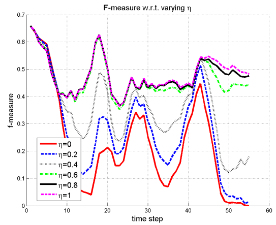
(b) F-measure
