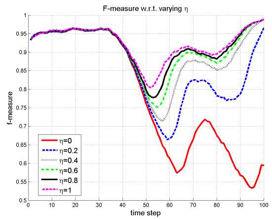
(b) F-measure
