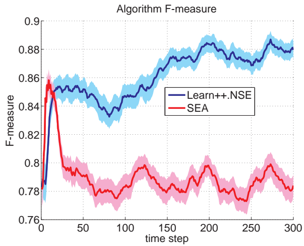
(c) F-measure
