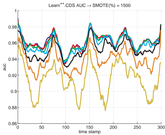
(e) SMOTE(%)=1500
