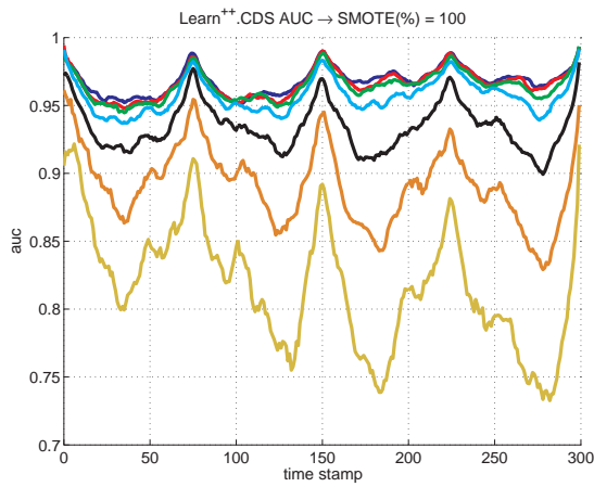
(a) SMOTE(%)=100
