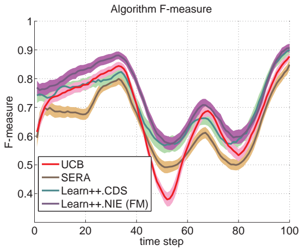
(c) F-measure
