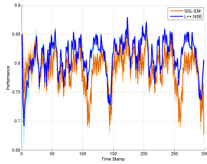
(a) Bias=0
