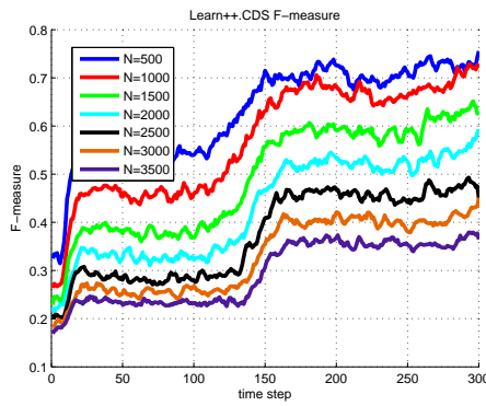
(c) F-measure
