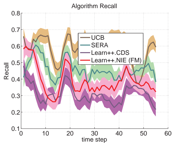
(e) Recall
