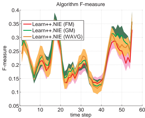
(c) F-measure
