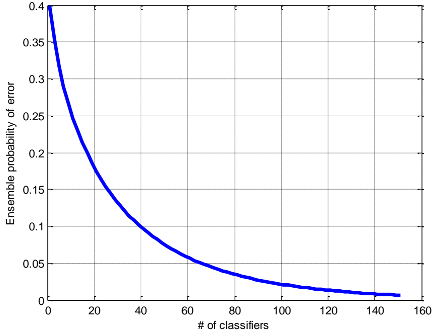
Fig. 2.5 : Theoretical error vs. the number of classifier for an ensemble combined using SMV. The error of each individual classifier is p = 0.4 and is computed using Eq. (2.6).
