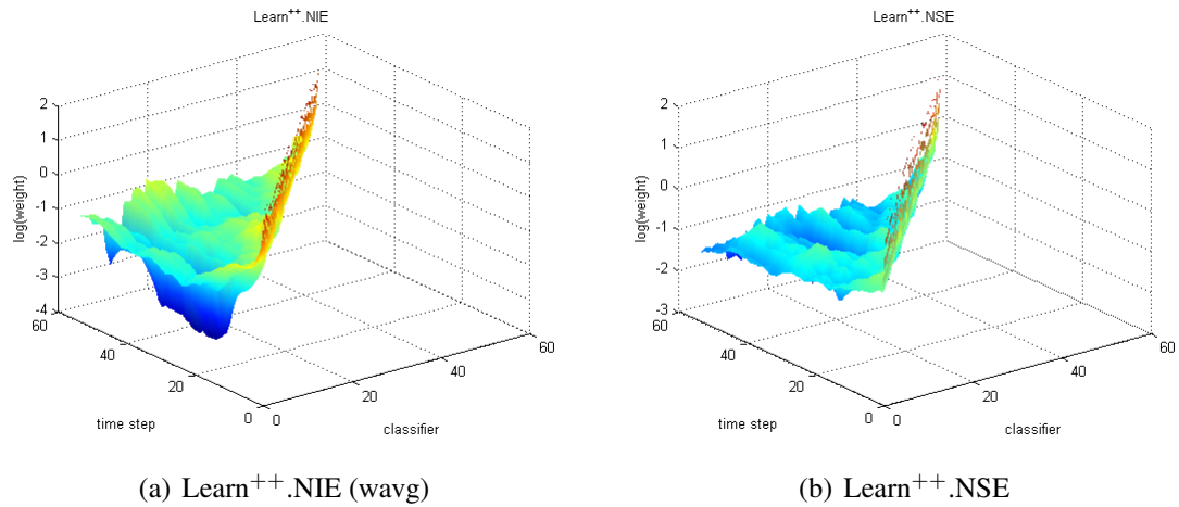
Fig. 5.32 : Learn ++ weight evolution on Elec2
