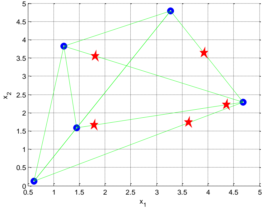
Fig. 3.9 : Demonstration of SMOTE sampling methods on synthetic data
