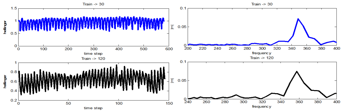
Fig. 5.33 : Distributional divergence measured between the 1 st batch and every subsequent batch of data in the entire NOAA databased (left). The FFT of the divergence (right) shows a large frequency component around 360 days.
