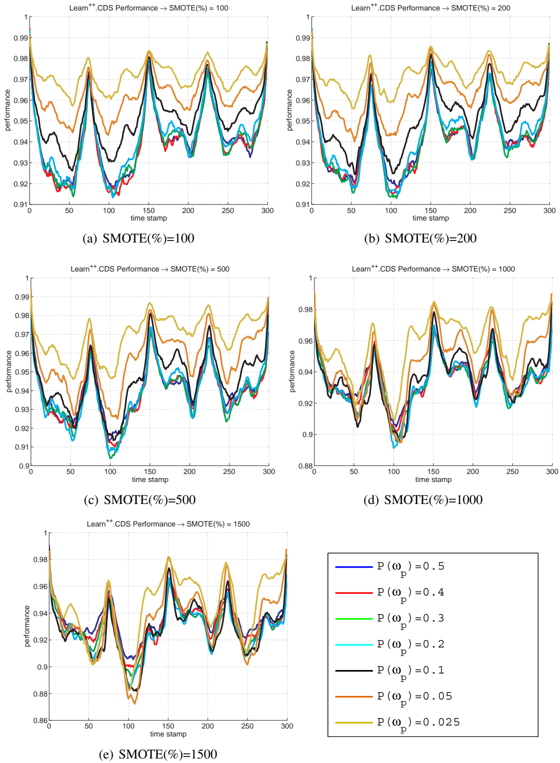
Fig. 5.7 : Raw Classification Accuracy for Learn ++ .CDS with varying levels of SMOTE
