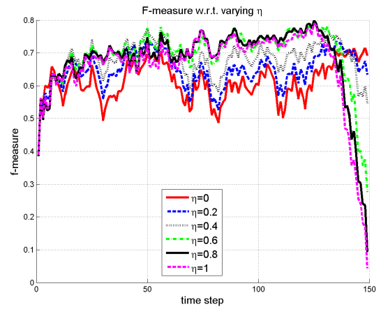
(b) F-measure
