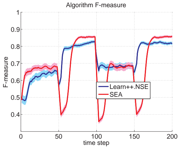
(c) F-measure
