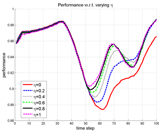
(a) Performance
