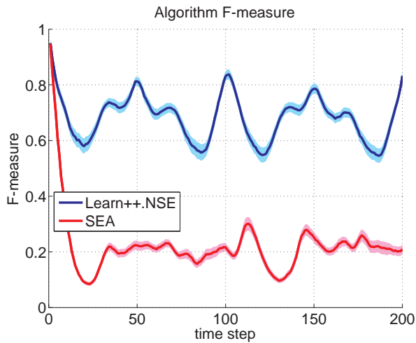
(i) F-measure
