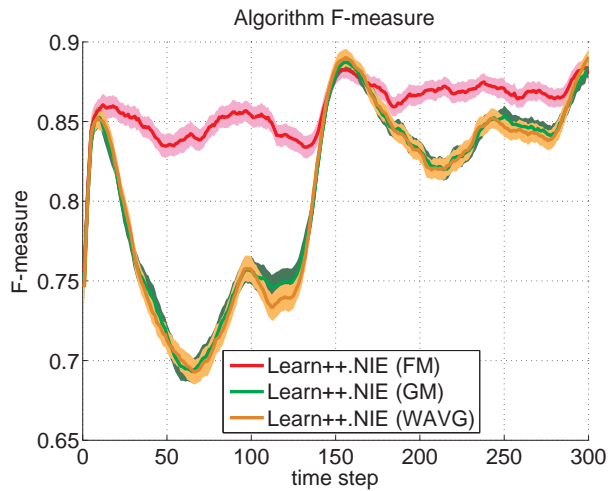
(c) F-measure
