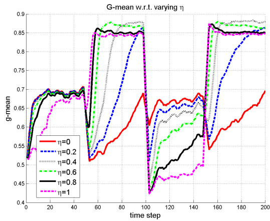
(c) G-mean
