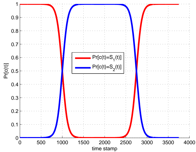
Fig. 2.4 : Probability of sampling from different sources under a gradual concept drift scenario with reoccurring environments
