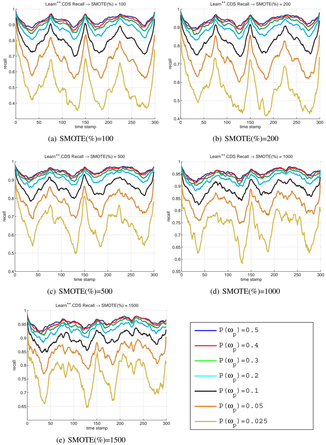
Fig. 5.6 : Recall for Learn ++ .CDS with varying levels of SMOTE
