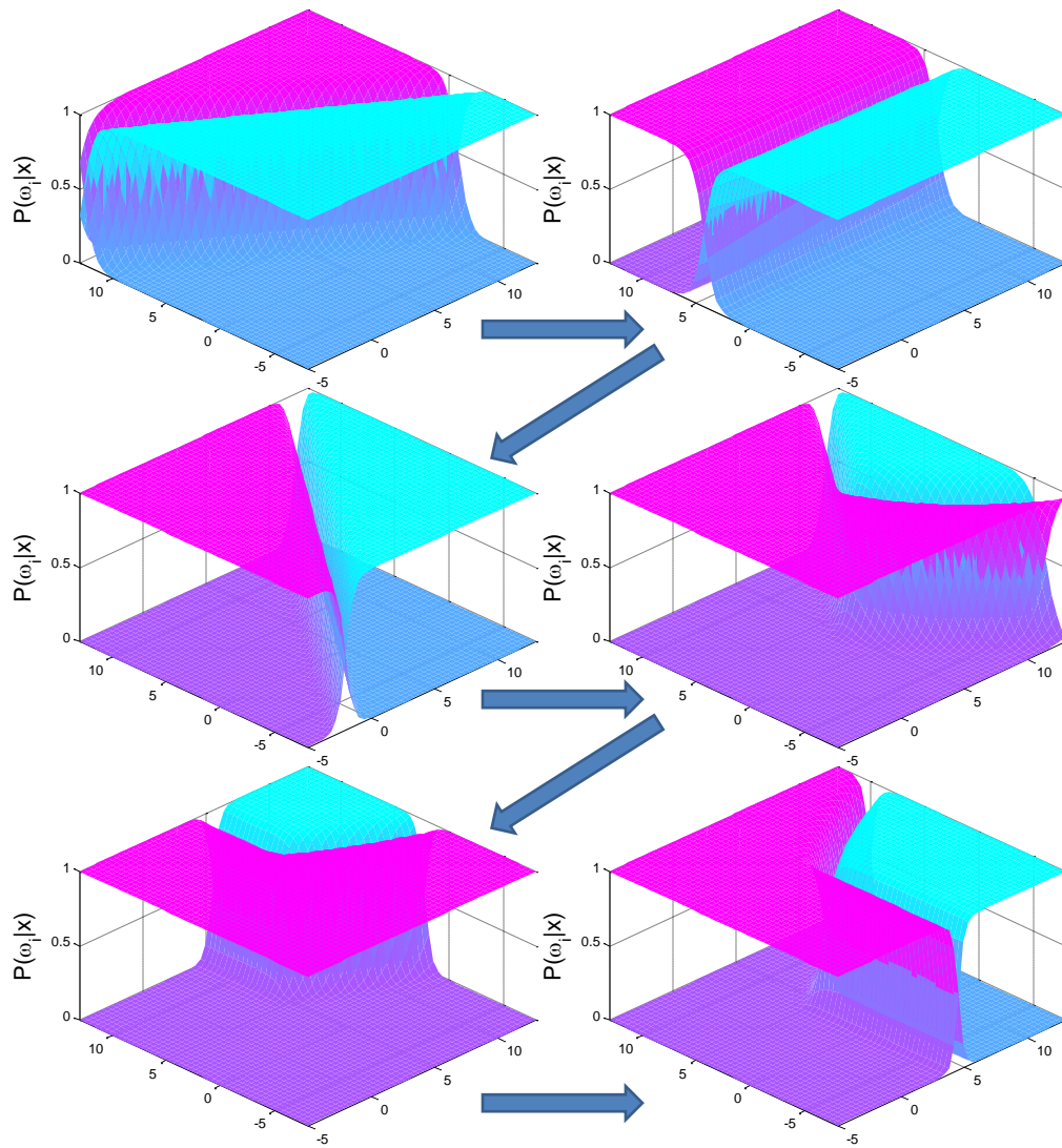
Fig. 5.45 : Evolution of the RandGauss dataset by observing the posterior probability. The dataset begins with 2-modes (one for each class) and begin slowly drifting. The drift stops at the third evolution point and remains static for 25 time stamps followed by the introduction of a new mode for the magenta class. The dataset continues to evolve with slow change followed by abrupt changes.
