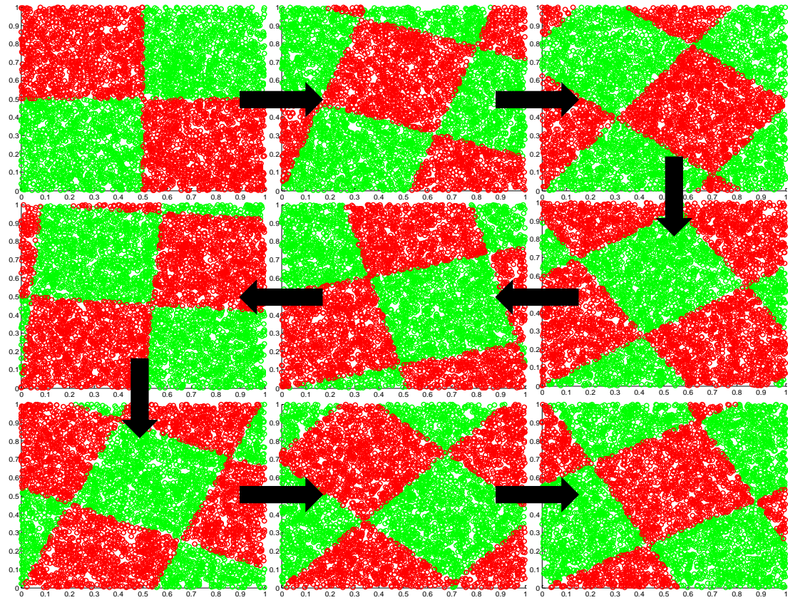
Fig. 5.43 : Evolution of the rotating checkerboard dataset
