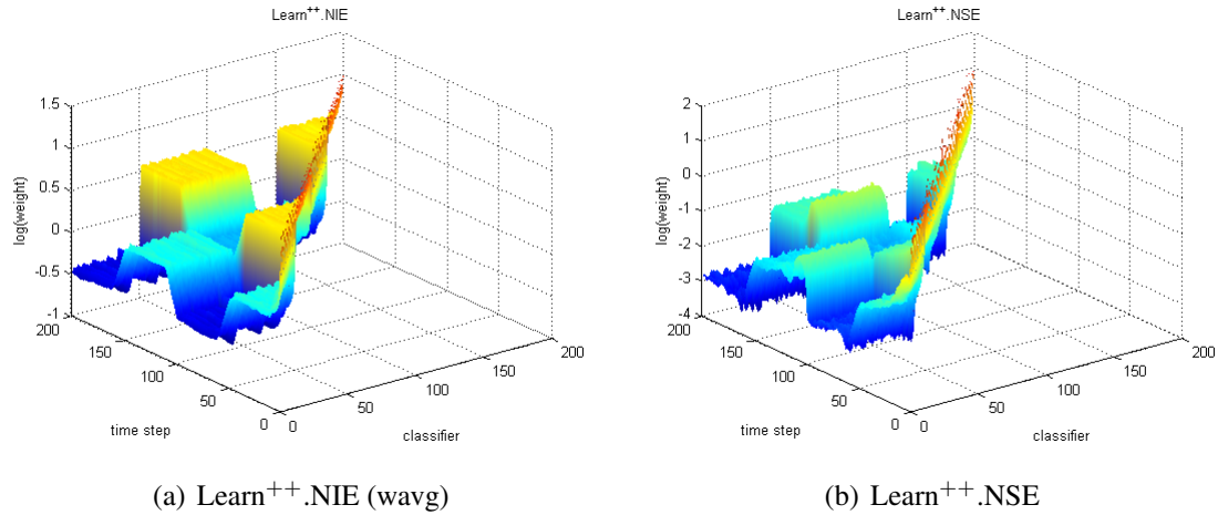
Fig. 5.27 : Learn ++ weight evolution on SEA
