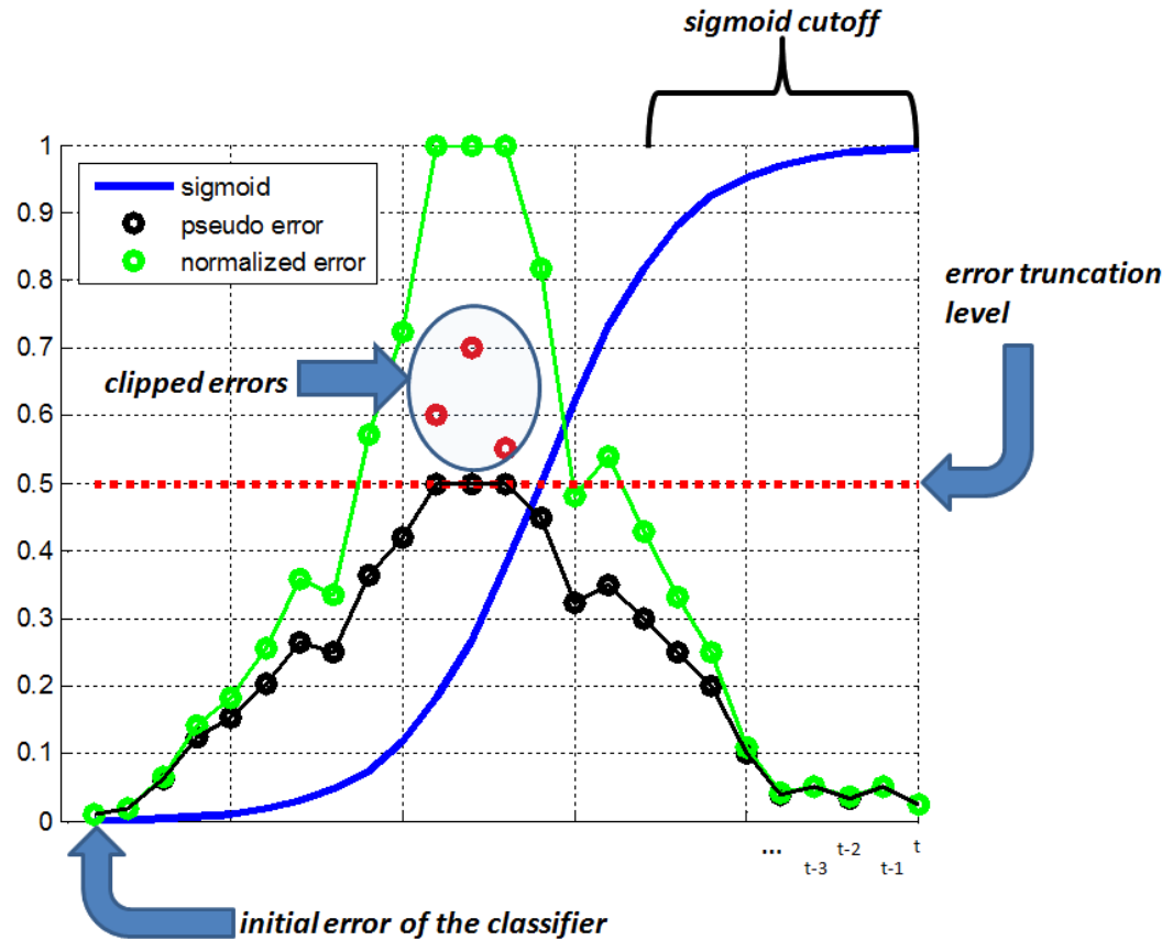
Fig. 3.19 : The more recent errors of a classifier are weighted heavier than errors ( \beta_k^{(t)} ) that have been committed a long time ago as indicated by the magnitude of the logistic function through time ( \sigma_k^{(t)} )
