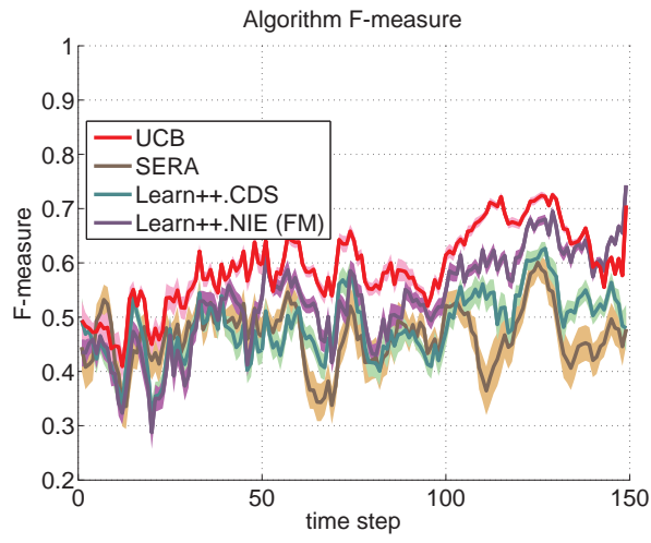
(c) F-measure
