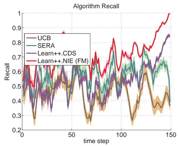
(e) Recall
