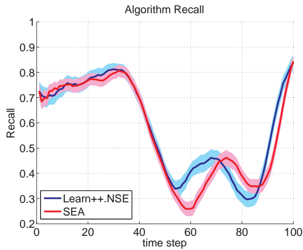
(e) Recall
