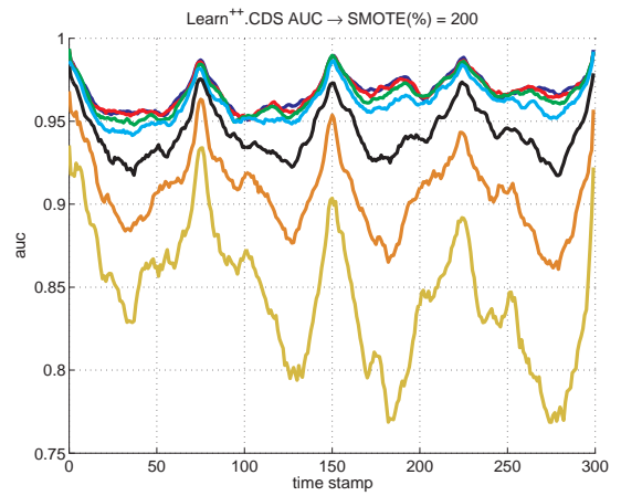
(b) SMOTE(%)=200
