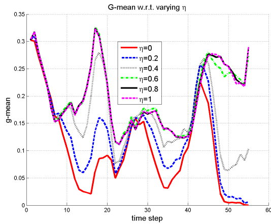
(c) G-mean
