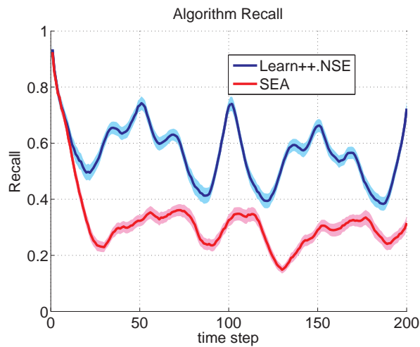
(k) Recall
