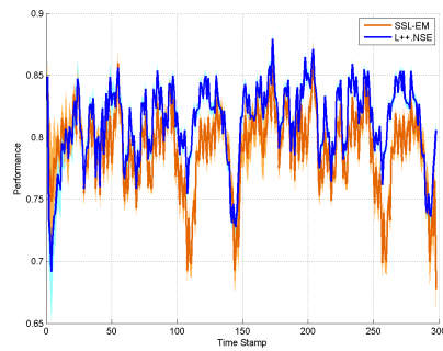
(c) Bias=3
