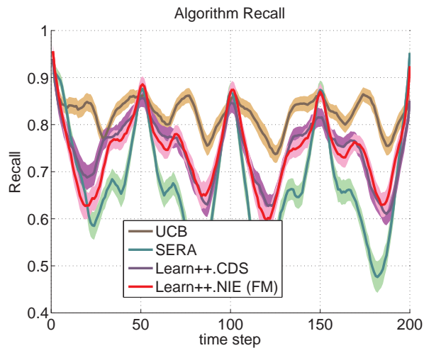
(e) Recall
