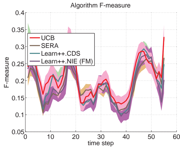
(c) F-measure
