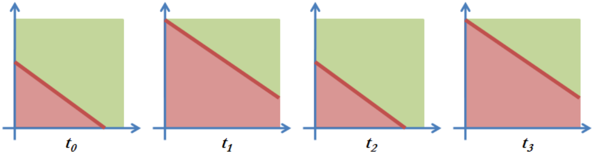
Fig. 5.23 : Demonstration of the shifting hyperplane problem presented by Street [49].
