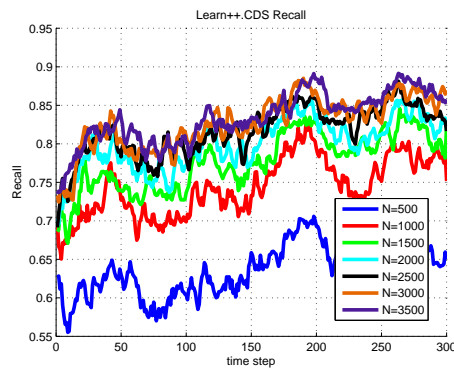
(e) Recall
