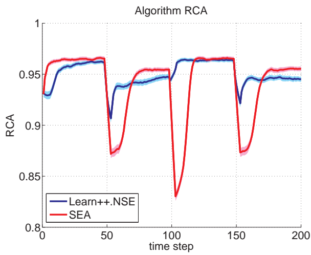
(a) Performance
