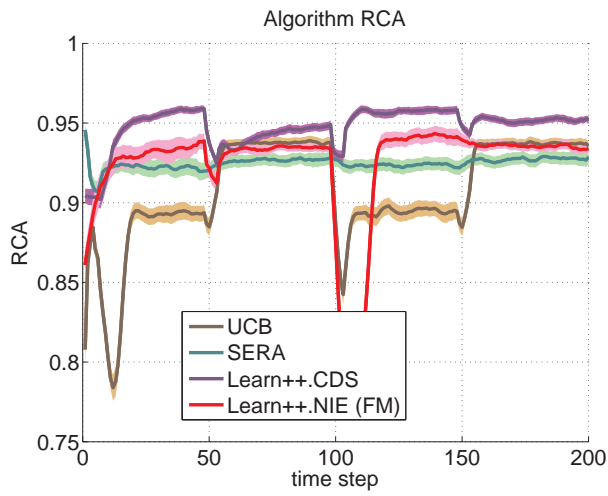
(a) Performance
