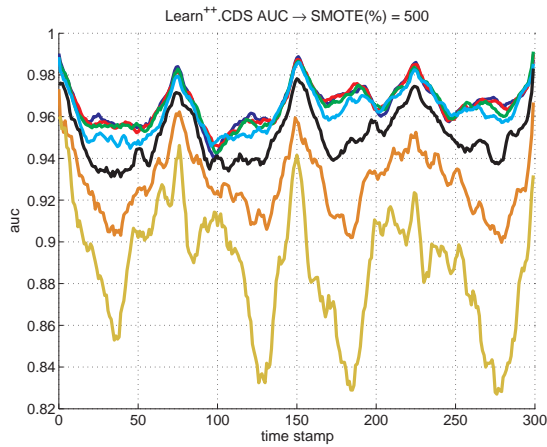
(c) SMOTE(%)=500
