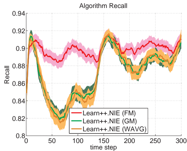
(e) Recall
