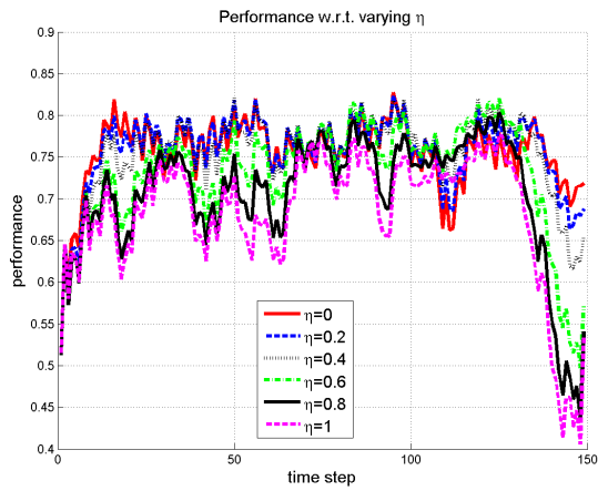
(a) Performance
