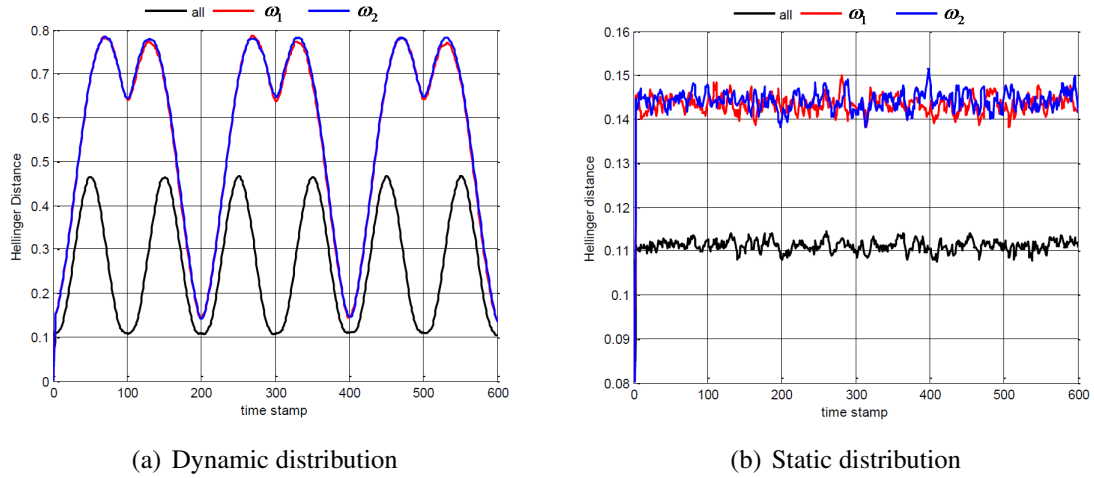
Fig. 4.7 : Hellinger distance computed on a rotating Gaussian centers problem. The Hellinger distance is computed between datasets \mathcal{D}_1 and \mathcal{D}_t where t = 2, 3, \dots, 600 for \omega_1 , \omega_2 , and all classes. Recurring environments occur when the Hellinger distance is at a minimum.
