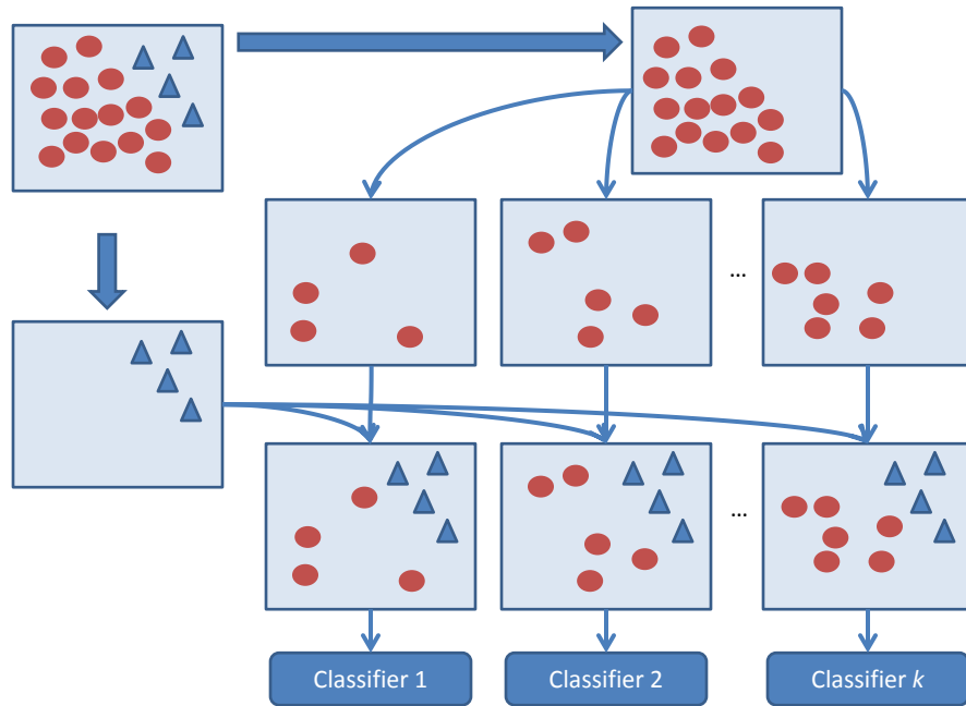
Fig. 3.12 : Disjoint set formulation used the bagging ensemble variation [101]. The majority class (red circles) are divided in disjoint sets and combined with the minority class (blue triangle) to form a new dataset used to generate a classifier.
